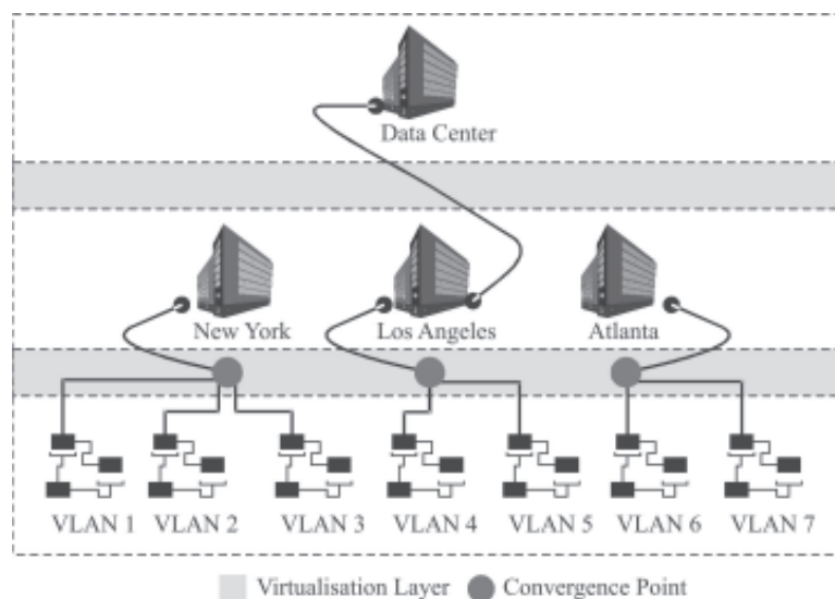
Fig. 26.2: Network Virtualization
